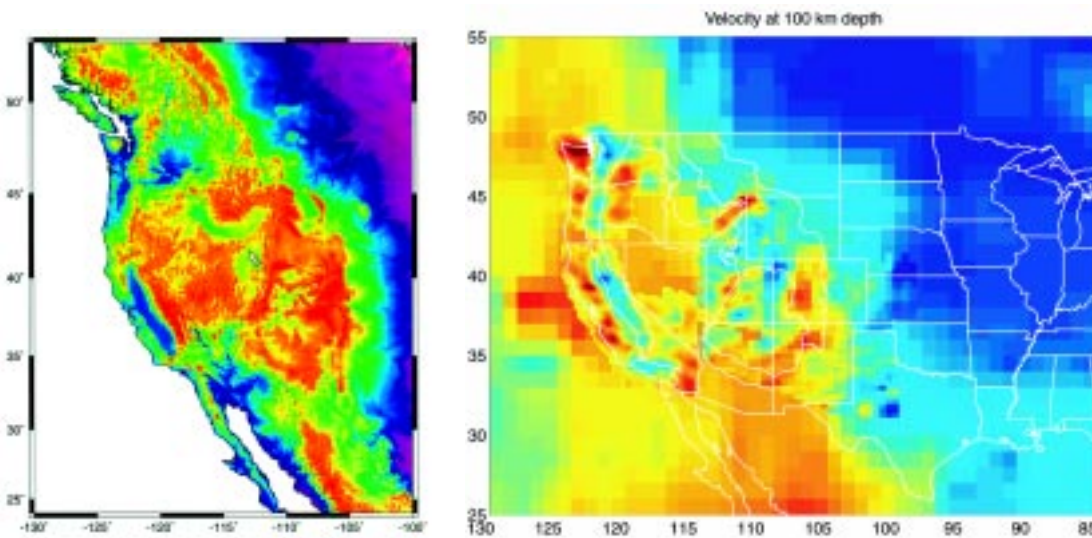
Figure 1b. Topography of western US filtered at 30 km wavelength (left). P-wave velocity structure at 100 km depth (from Dueker and Humphreys, 19xx; right). Linear Sierra Nevada/ Great Valley structures are colinear with mantle anomalies. The mantle beneath the Snake River Plain and Yellowstone hotspot is slow, while the Colorado Plateau has relatively fast mantle ringed by low velocities in the basin and range and Rio Grande rift system.
