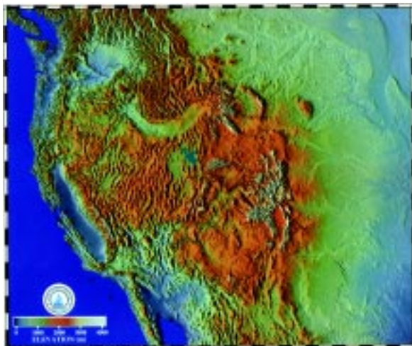
Figure 1c. Topography of Western US filtered at 1 km wavelength (Simpson and Anders, 1992). Many structures, marking extension, volcanoes in the Pacific northwest, a crustal welt marking the Mendocino Triple Junction, the track of the Yellowstone hotspot.
